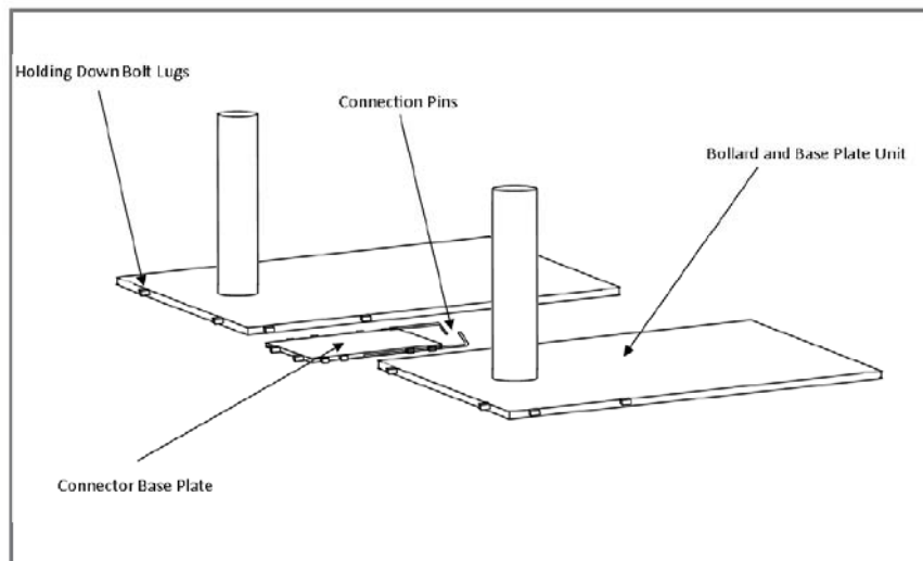
Linking multiple bollards to form a continuous barrier.
